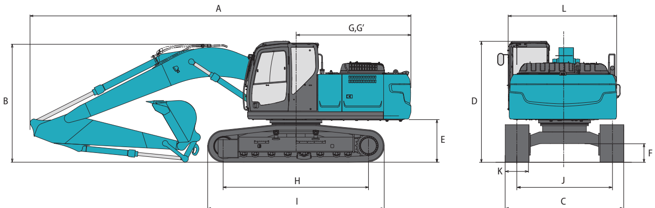
SK210LC/SK210NLC
