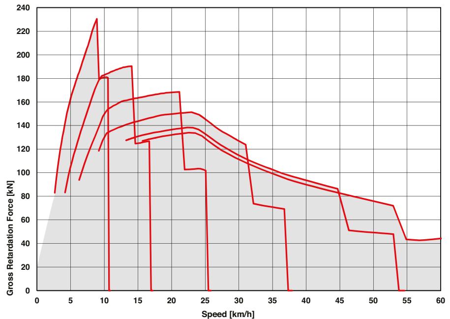
ADT, B30E 6X6, Tier 4f - Retardation
