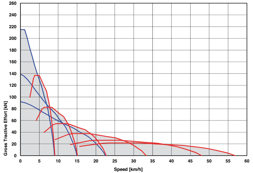
ADT, B30E 6x6, Tier 4f - Tractive Effort
